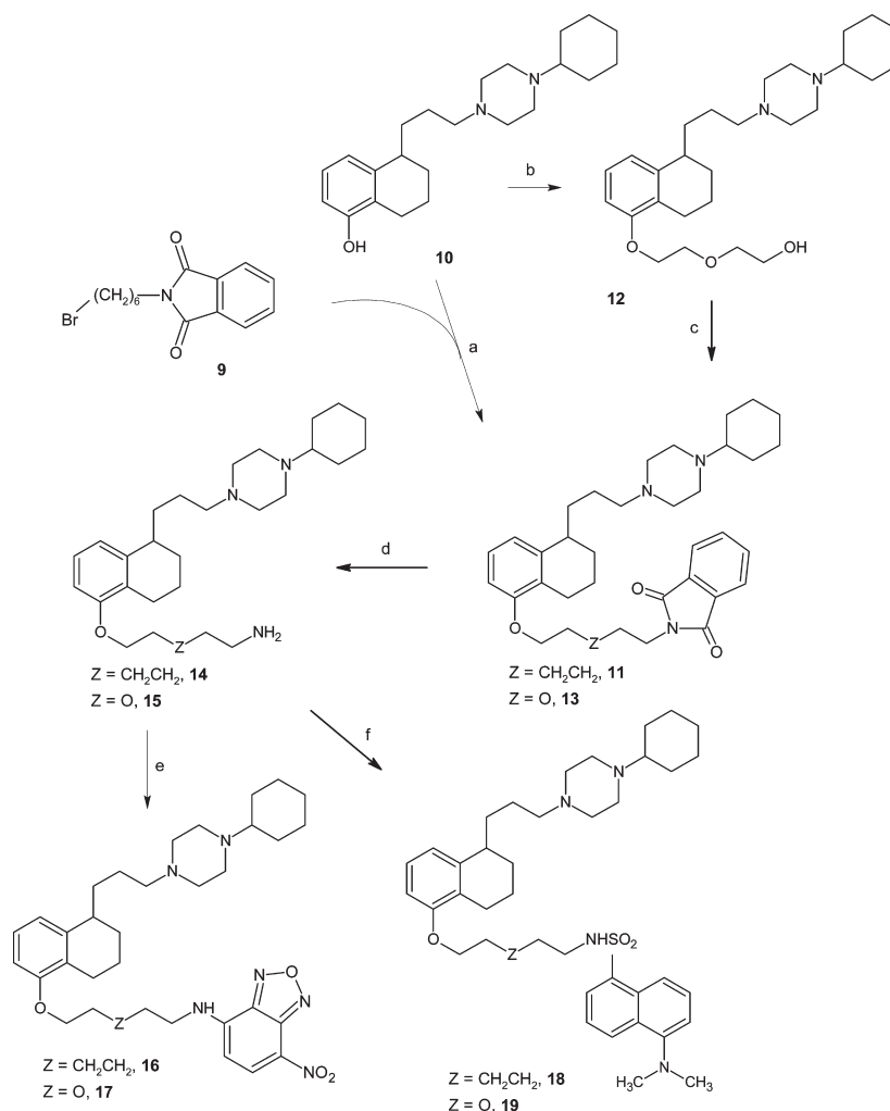
Scheme 2. Synthesis of Fluorescent Compound 1 Analogues: Fluorescent Tag at the Tetralin Nucleus a
