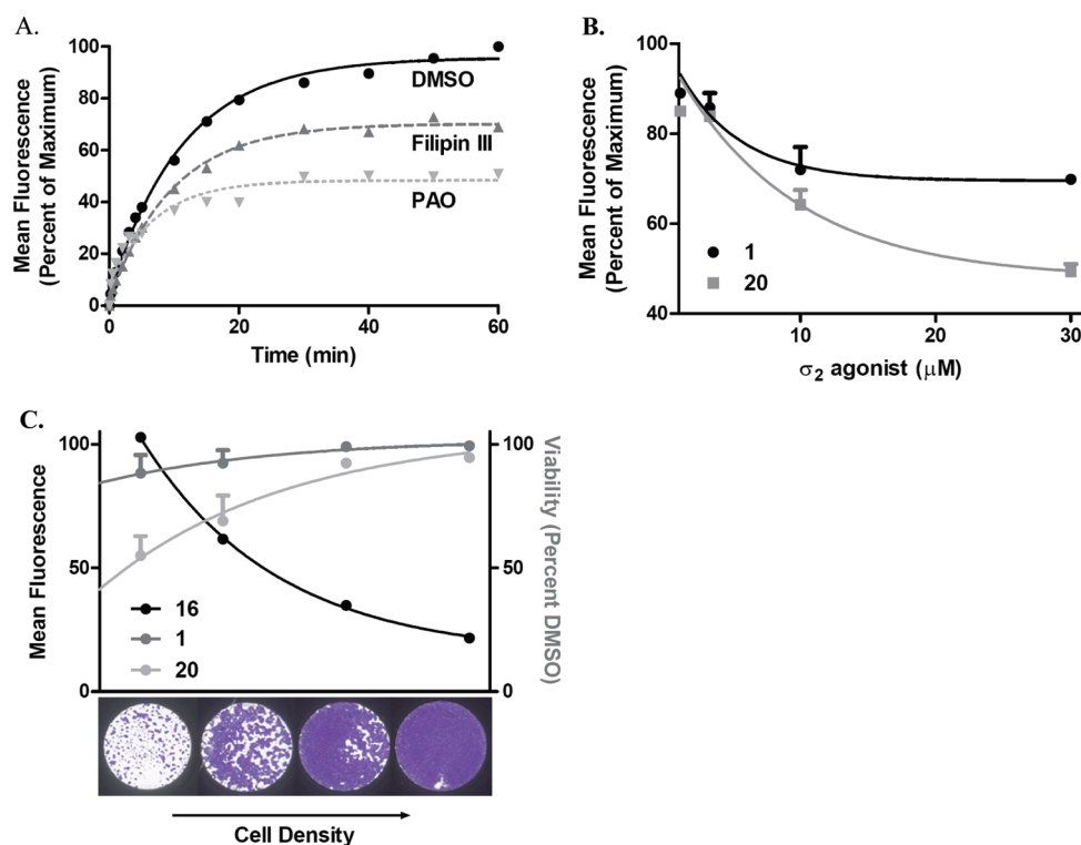
Figure 1. Cellular internalization of the fluorescent \sigma_2 receptor ligand 16: BxPC3 pancreatic cancer cells were treated for 1 h with the endocytosis inhibitors Filipin III (5 \mu\text{g}/\text{mL} ) or phenylarsine oxide (PAO, 10 \mu\text{M} ) or DMSO vehicle for 60 min prior to kinetic uptake analysis of 16 (25 nM) by flow cytometry. Compound 16 uptake represents the percentage of the mean fluorescence of maximum signal intensity. (B) Competition of compound 16 by \sigma_2 agonist structural analogues. BxPC3 cells were treated with increasing doses of compounds 1 or 20 for 45 min prior to replacement with compound 16 (25 nM) for 45 min and fluorescence intensity quantified by flow cytometry. (C) Cell density dependence \sigma_2 agonist uptake and cell death. BxPC3 cells were seeded at increasing densities to achieve a range of dividing, subconfluent and quiescent, confluent cultures. The following day, cells were treated with compound 16 (25 nM) and fluorescence intensity quantitated by flow cytometry. Alternatively, cell were treated with compound 1 or 20 (100 \mu\text{M} ) for 24 h and viability compared to DMSO control.
